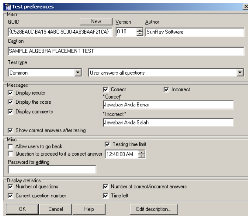
Gambar 6 Test Preference
