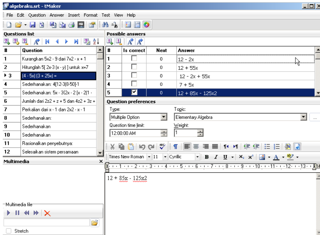
Gambar 3 tMaker
