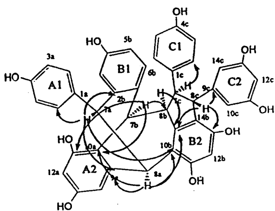
Fig 1 Significant HMBC (H→C) correlation of 1
