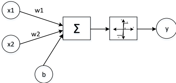
Gambar 4. Model Jaringan Perceptron
